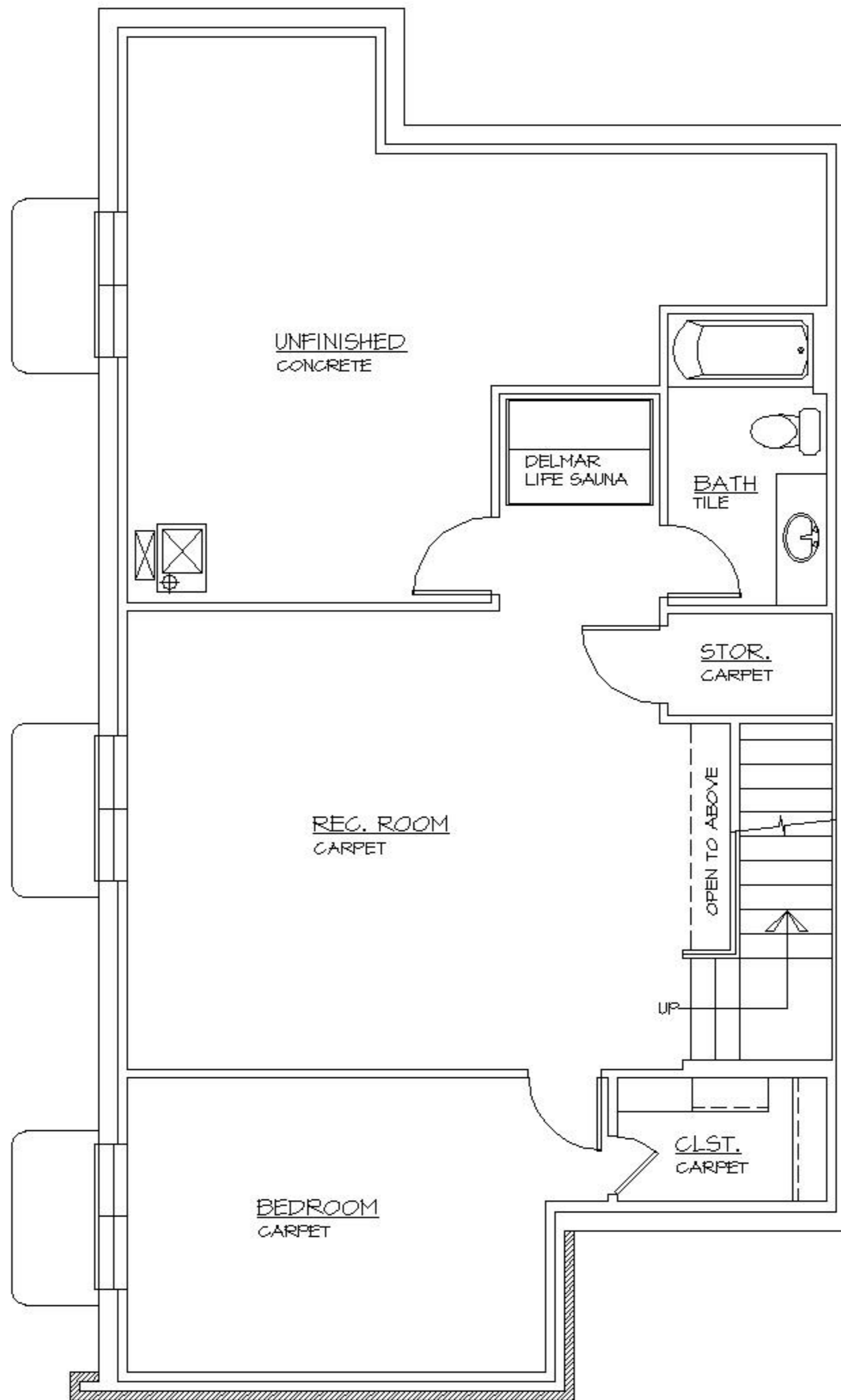
BASEMENT FLOOR PLAN 771 SQUARE FEET FINISHED
